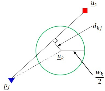
Fig. 4. Non-LoS identification at the j^{\text{th}} beacon.
